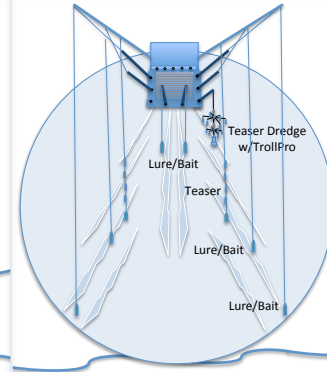
Basic Set-Up for TrollPro in Multi-tiered Teaser Dredge
